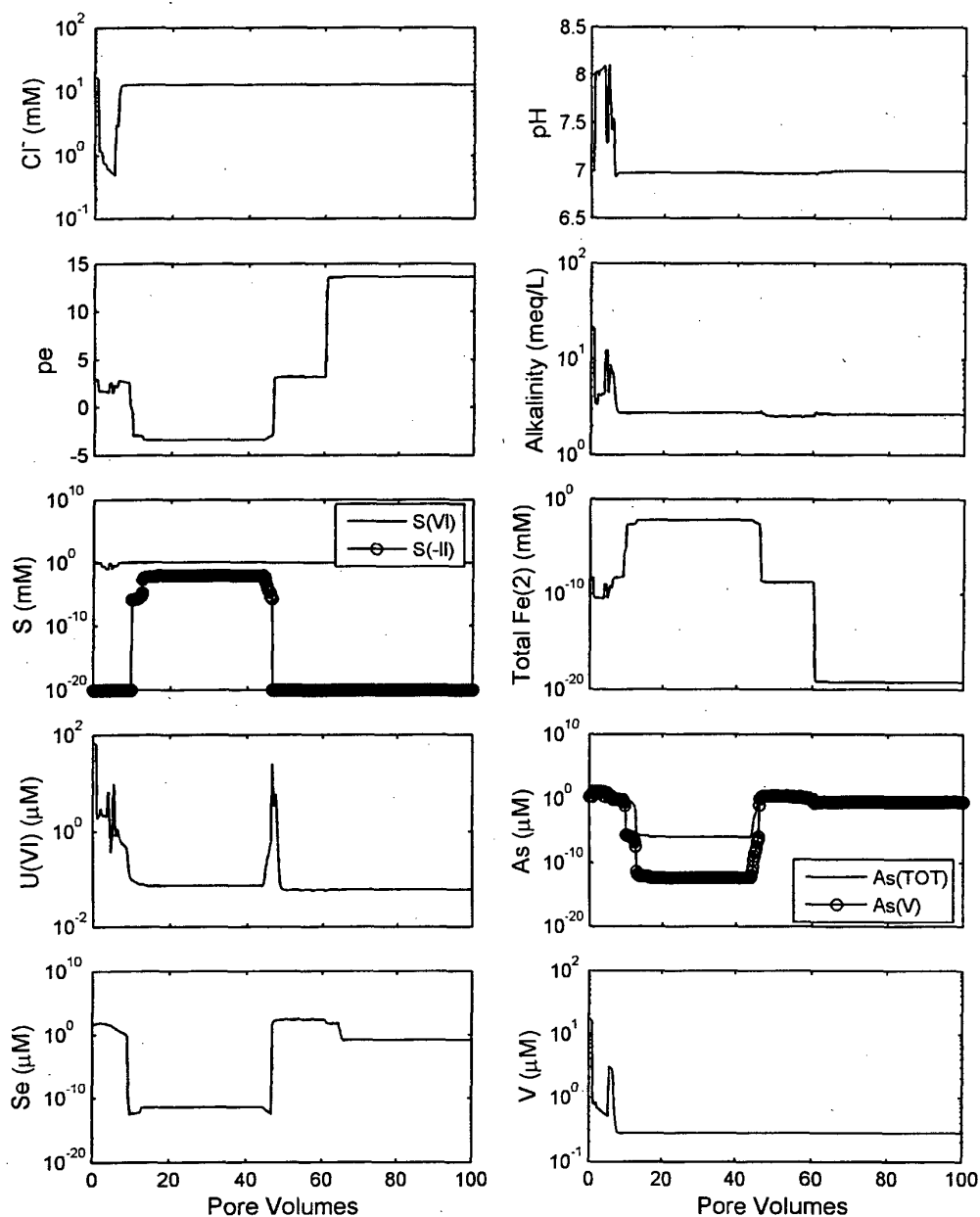
Figure 28. Simulation 11 results. Mass transfer coefficient changed to 10^{-2} . Oxic influent groundwater. Calcite, goethite, and elemental Se (50 ppm) initially present. 265 mg/L of H_2S(g) added to the influent water during pore volumes 3.0 to 3.6. Pyrite and uraninite precipitation not allowed. Amorphous FeS and UO_2 precipitation allowed. Sulfide concentration indicated at 1 \times 10^{-20} M is actually \leq 1 \times 10^{-20} M in plot.
