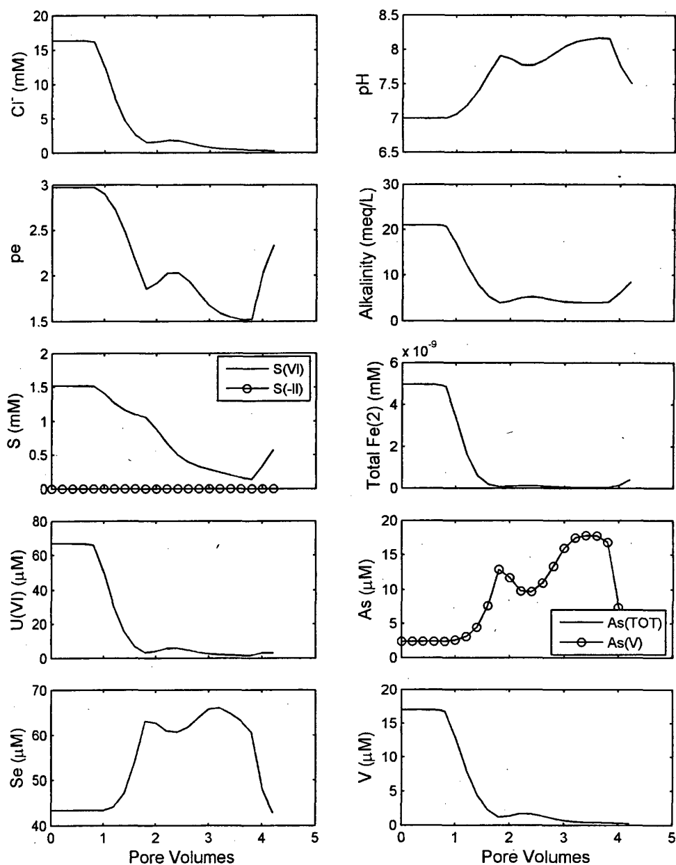
Figure 21. Simulation 10 results. Oxic influent groundwater. Calcite, goethite, and elemental Se (50 ppm) initially present. 265 mg/L of \text{H}_2\text{S}(\text{g}) added to the influent water during pore volumes 3.0 to 3.6. Pyrite and uraninite precipitation not allowed. Amorphous \text{FeS} and \text{UO}_2 precipitation allowed. Mass transfer coefficient = 10.
