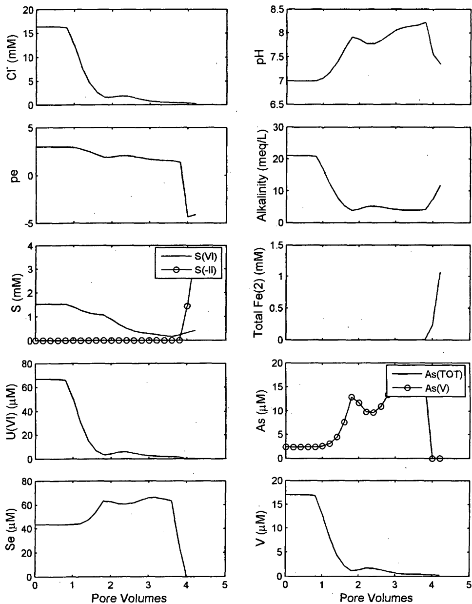
Figure 19. Simulation 8 results. Oxidic influent groundwater. Calcite, goethite, and elemental Se (50 ppm) initially present. 265 mg/L of \text{H}_2\text{S(g)} added to the influent water during pore volumes 3.0 to 3.6. Pyrite precipitation not allowed. Elemental sulfur precipitation allowed. Mass transfer coefficient = 10.
